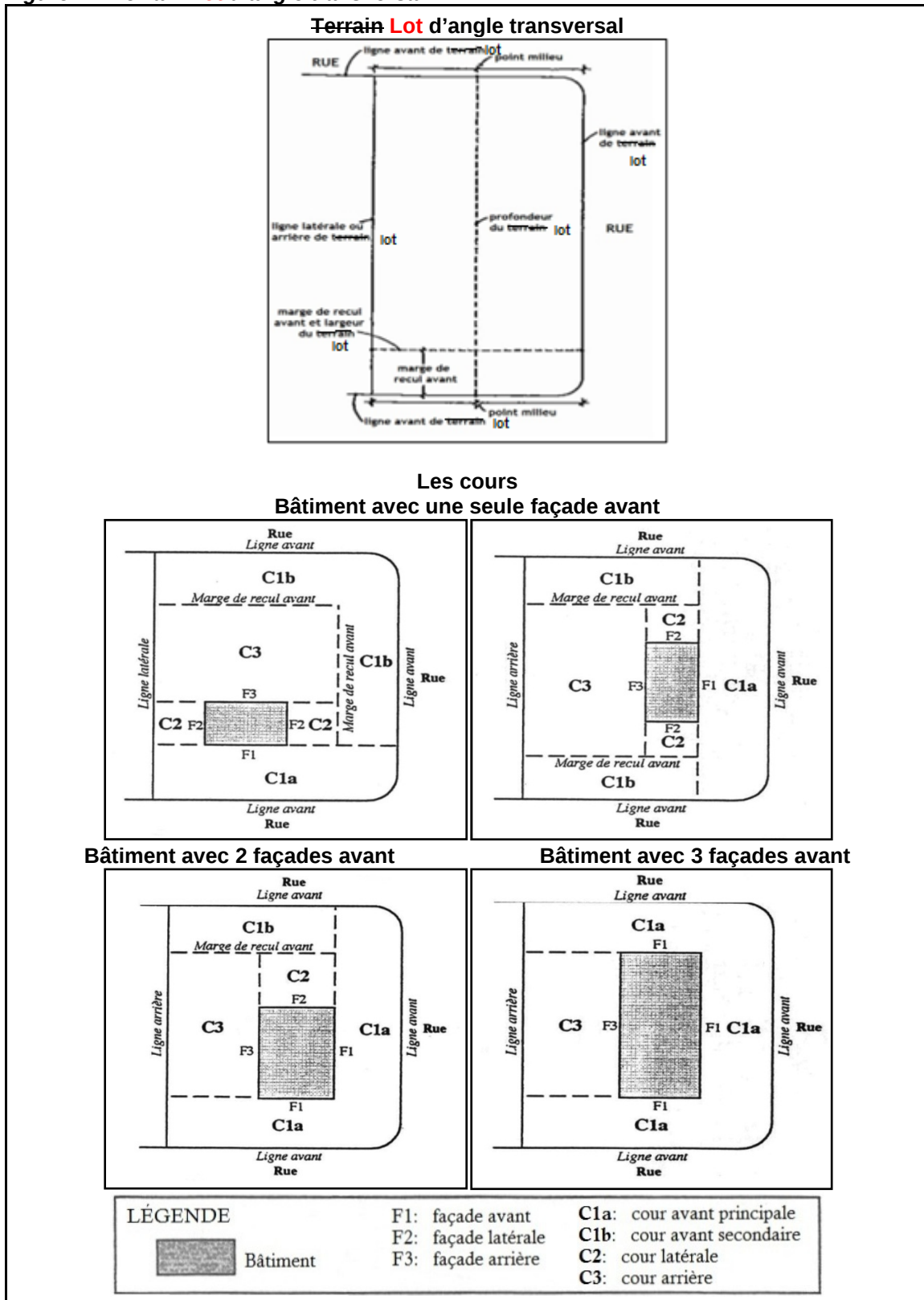
Figure 11 Terrain Lot d'angle transversal
